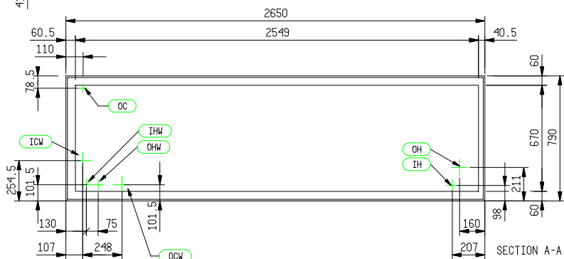
PIPES POSITIONS FOR FRONTAL AIR SUCTION VERSION
