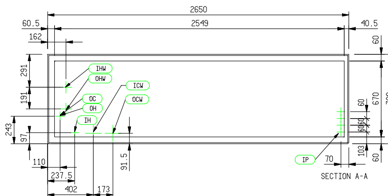
PIPES POSITIONS FOR REAR/BOTTOM AIR SUCTION VERSION
